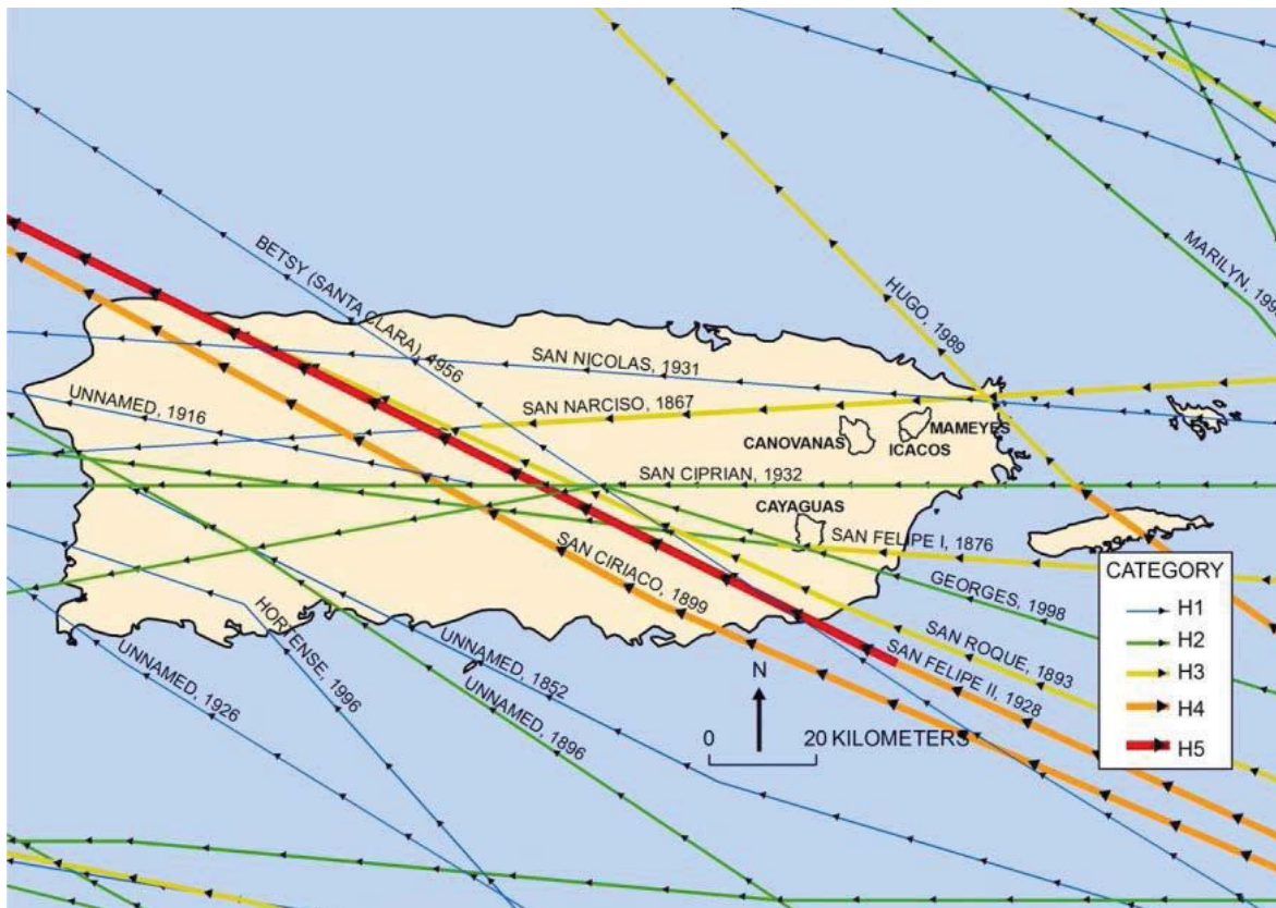
FIGURE 1-3. HISTORICAL STORM TRACKS IN PUERTO RICO
